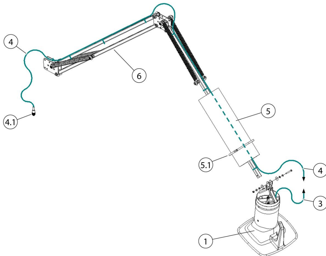
Fig.14 : Cable routing – extraction arm 2–4 metres
