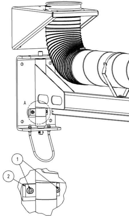
Fig.11 : Brake on the extension arm
