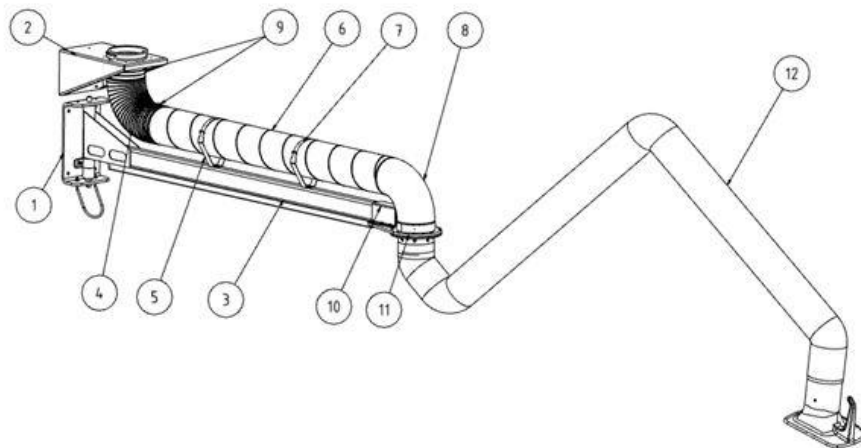
Fig.3 : Boom arm with extraction arm
