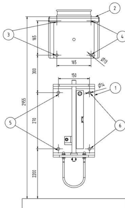
Fig.4 : Wall bracket
