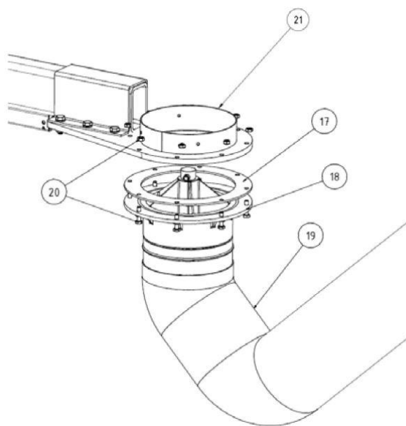
Fig.9 : Extraction arm on the extension arm
