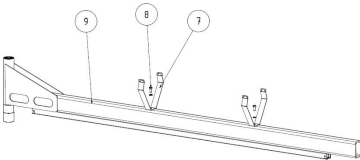
Fig.5 : Pipe bracket and extraction arm mounting bracket
