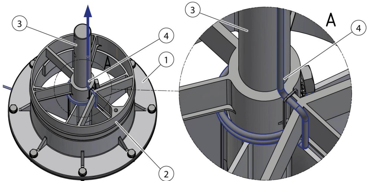
Fig.12 : Slewing ring
