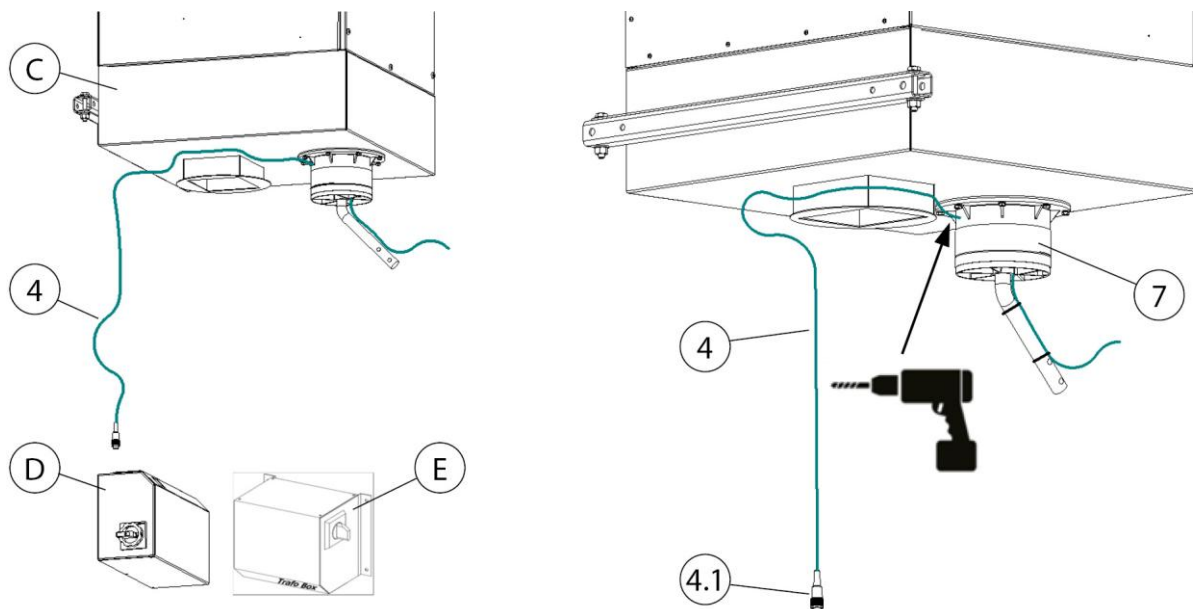
Fig. 15: Cable laying – stationary unit
