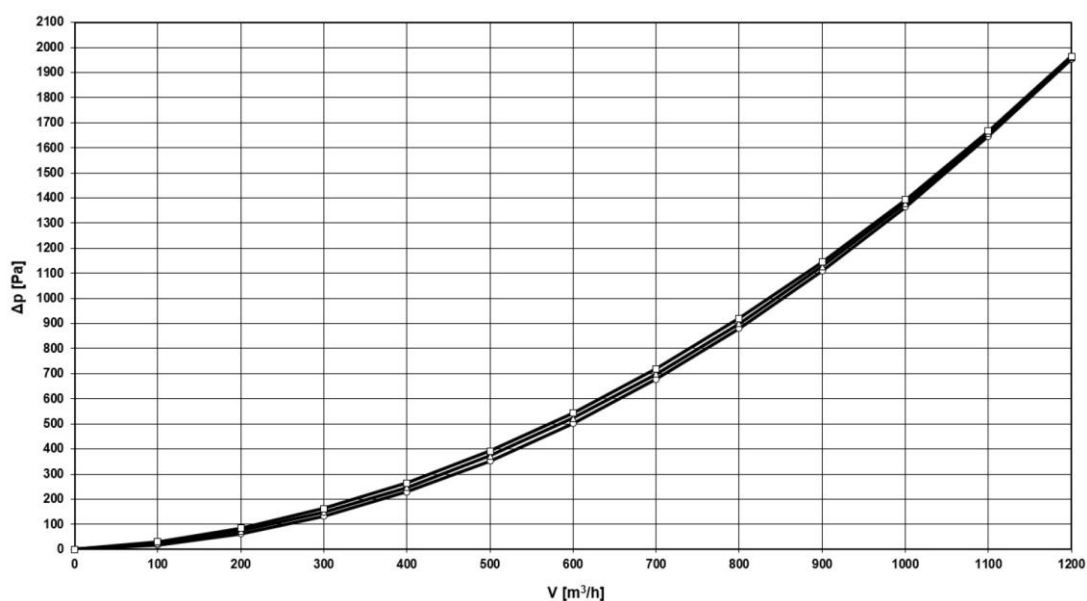
Fig. 17: Pressure Loss Diagram
