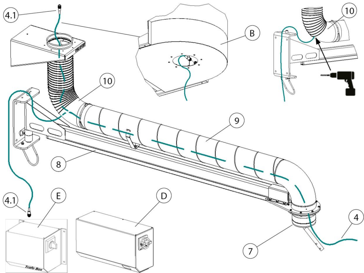
Fig. 13: Cable routing – extraction arms with crane cantilever
